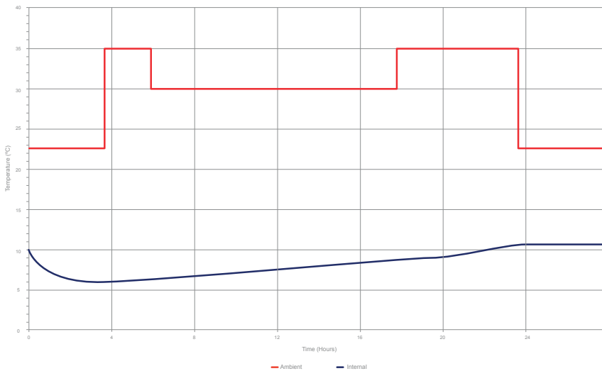
Series 4 - 424, Unit 1, ISTA Summer Thermal Performance (Control Set: ISTA 7D Summer Profile, No Payload, -18°C to 2°C TIC Conditioning, No TIC Staging) Source: MTS Lab 14 April 2014
